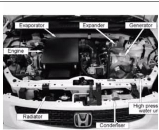
Waste heat utilization in Honda car
