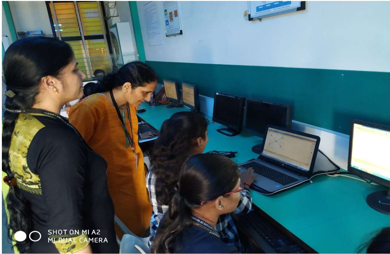
Packet Tracer
